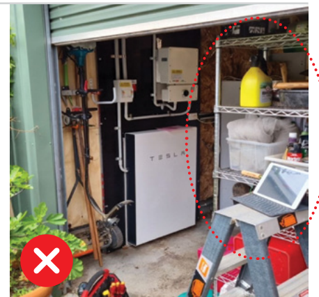
Figure 1.1: Non-fixed shelving is not adequate mechanical protection for a battery system installed in an area accessible to cars.
